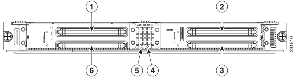
Figure 2-5 Cisco ASR 1000 Series SIP Faceplate
